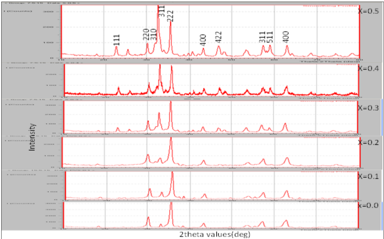
Figure 1 XRD Pattern of Sm substituted Ni Cd nano Ferrite
