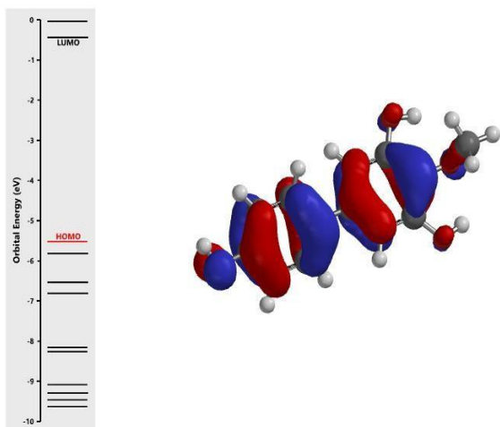
5(4-hydroxyphenyl)-3-hydroxy-2-methoxyphenol (HOMO)
