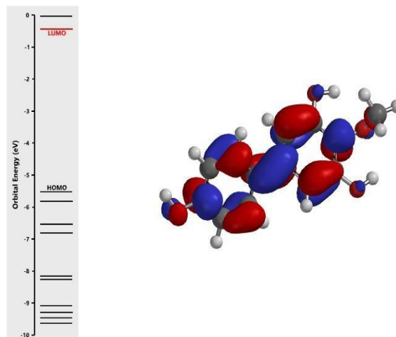
5(4-hydroxyphenyl)-3-hydroxy-2-methoxyphenol (LUMO)
