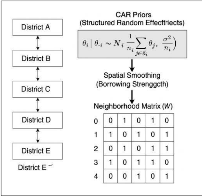
Figure 2 Diagram of spatial correlation via CAR priors and neighborhood matrices
