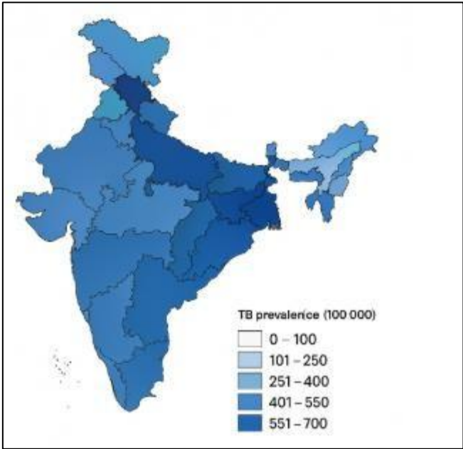
Figure 4 Example map of small-area estimates for TB prevalence using BHM. [18]
