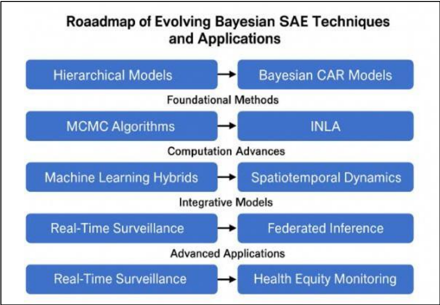
Figure 5 Roadmap of evolving Bayesian SAE techniques and applications.
