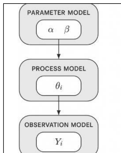
Figure 1 Schematic of the Bayesian hierarchical structure for small-area estimation
