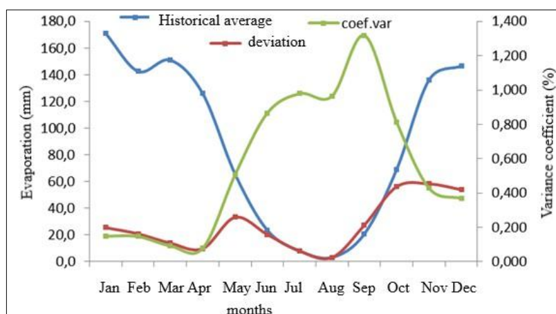
Figure 24 Distribution of monthly evaporation and its values between the municipalities of Sebastião Leal and Uruçuí – PI; Source: Medeiros, 2022.
