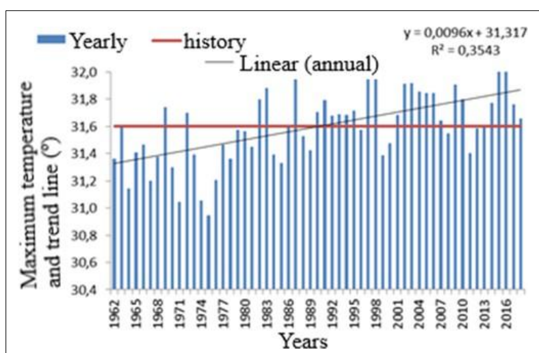
Figure 3 Distribution of annual maximum temperature, historical average and trend line between the municipalities of Sebastião Leal and Uruçuí do Piauí in the period 1962-2018; Source: Medeiros, 2022.
