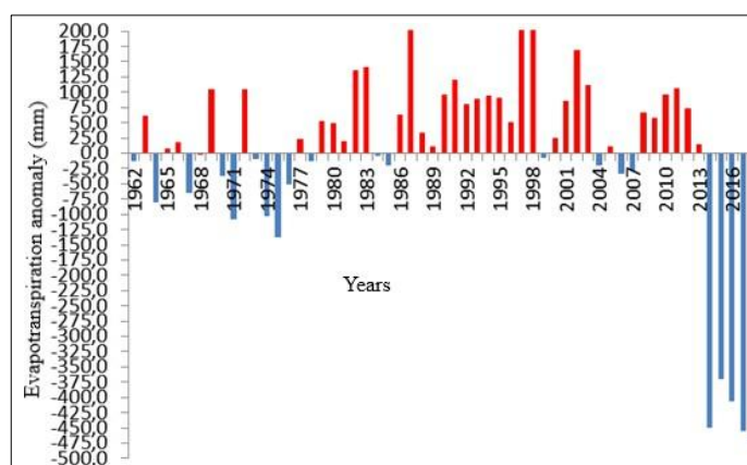
Figure 19 Distribution of the annual evapotranspiration anomaly between the municipalities of Sebastião Leal and Uruçuí do Piauí in the period 1962-2018; Source: Medeiros, 2022.
