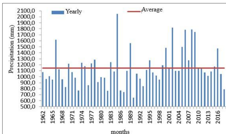
Figure 15 Representability of annual rainfall rates and historical average between the municipalities of Sebastião Leal and Uruçuí do Piauí in the period 1962-2018; Source: Medeiros, 2022.
