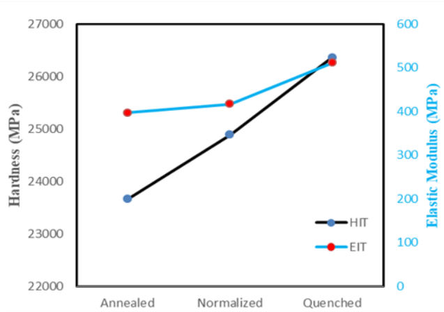
Figure 4 Instrument Hardness ( H_{IT} ) and Elastic Modulus ( E_{IT} ) variation for TiN films
