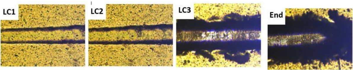
Figure 6 (a) Optical view of critical loads (LC1, LC2 & LC3) and end of scratch for TiN film on Annealed substrate
