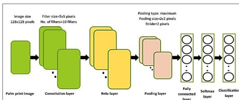
Figure 7 The architecture of the PCNN system[3]
