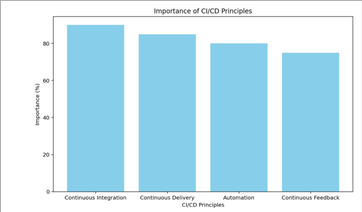
Figure 3 CI/CD Principles
