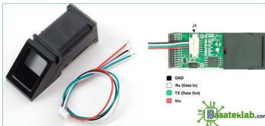
Figure 5 R305 fingerprint sensor and its pin connection
