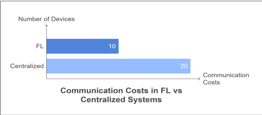
Figure 6 Privacy Mechanisms
