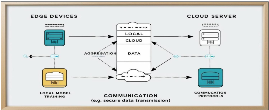
Figure 2 Simulation Workflow
