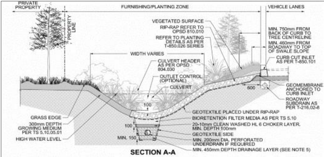
Figure 1 A cross-sectional diagram of a typical bioswale, detailing its structural components
