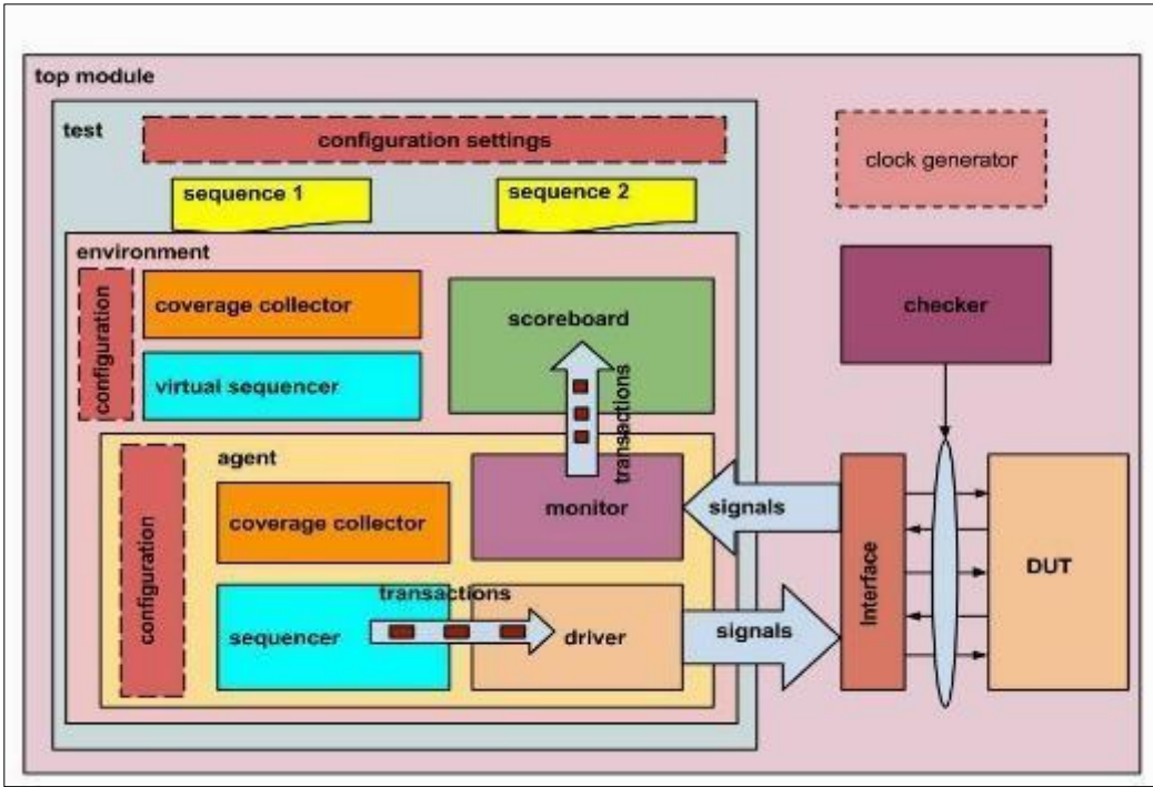
Figure 5 UVM Environment Components
