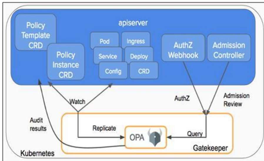
Figure 8 Managing Policies on Kubernetes using OPA Gatekeeper
