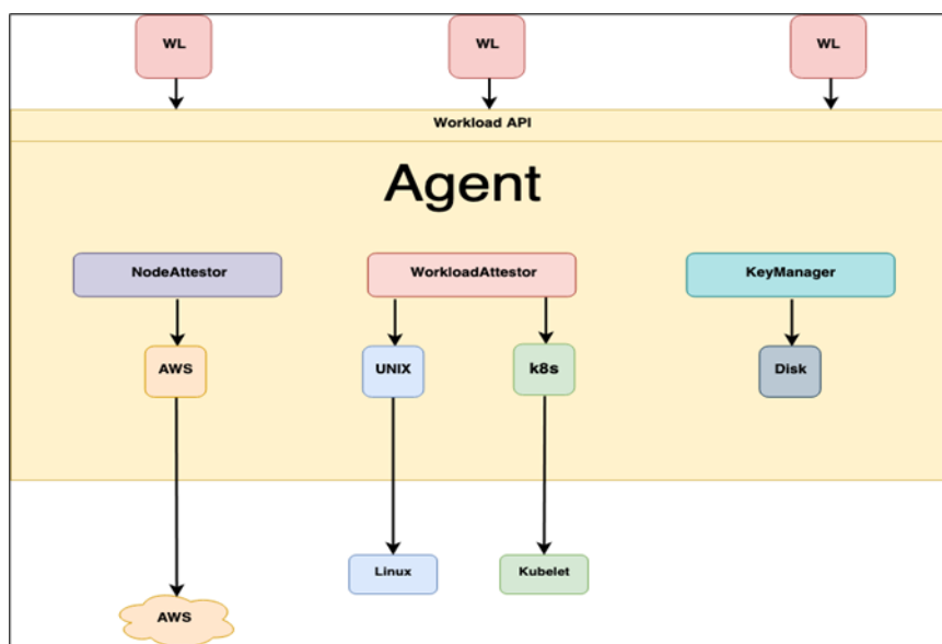
Figure 7 Some of SPIRE Concepts
