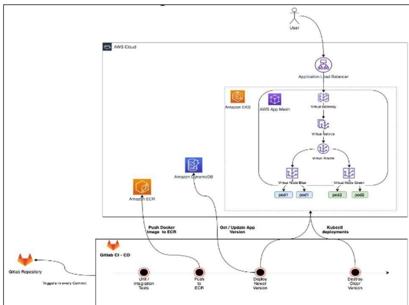
Figure 2 CI/CD with Amazon EKS using AWS App Mesh and Gitlab
