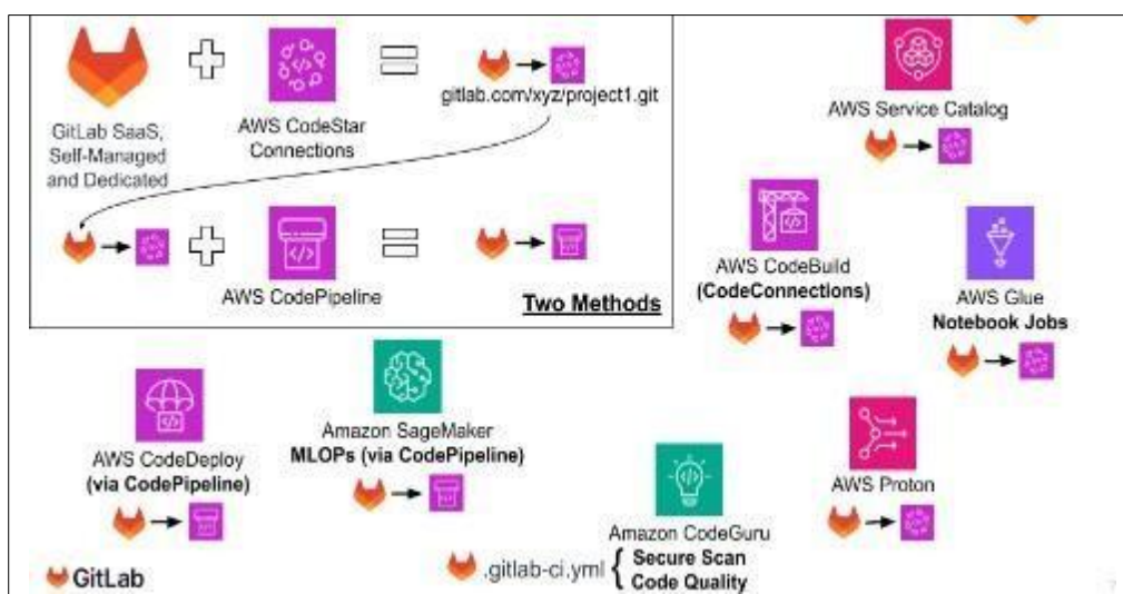
Figure 8 Ultimate guide to migrating from AWS CodeCommit to GitLab
