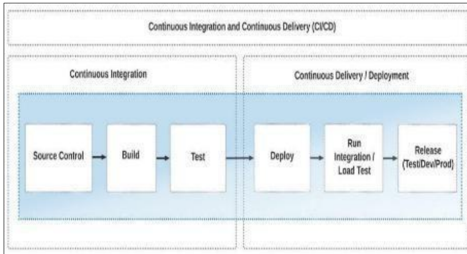
Figure 11 CI/CD for Cloud-Native Applications
