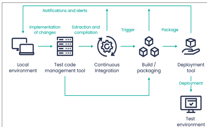
Figure 3 Automating CI/CD continuous integration & continuous delivery
