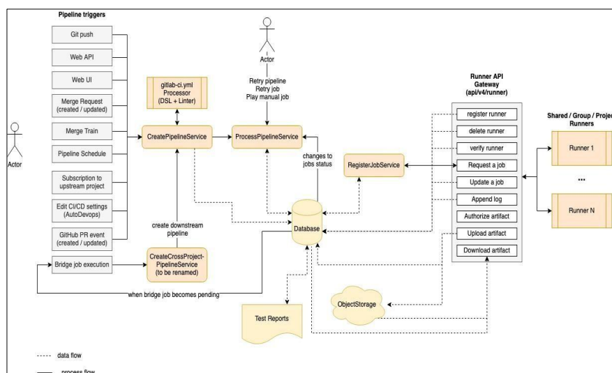
Figure 6 CI/CD development guidelines
