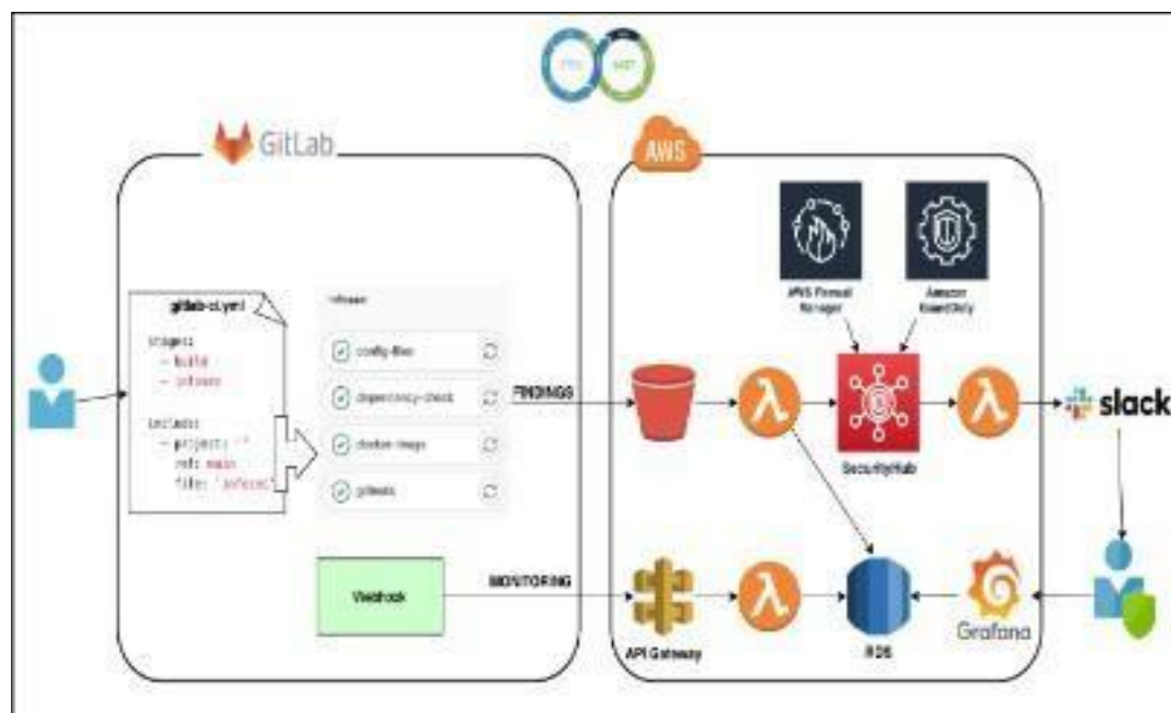
Figure 4 Incorporating security in CI/CD pipelines
