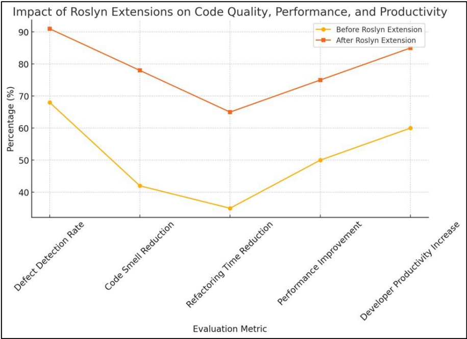
Figure 3 A line graph showing the impact of Roslyn Extensions on code quality, performance, and developer productivity
