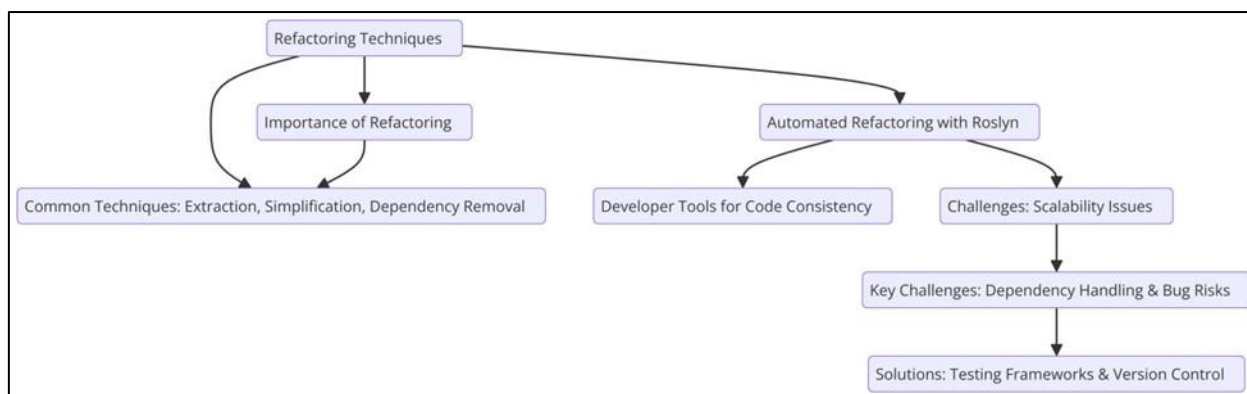
Figure 2 Image illustrating the role of refactoring in improving software maintainability, reducing technical debt, and ensuring adaptability. The diagram highlights key techniques, automation through Roslyn, developer tools, scalability challenges, and solutions such as testing frameworks and version control
