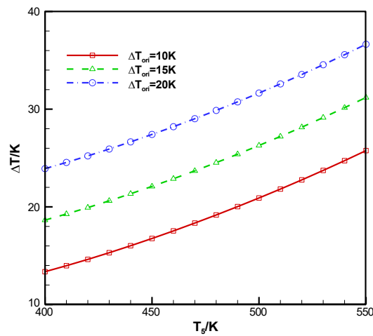
Figure 7 Variation of minimum temperature difference with T_5
