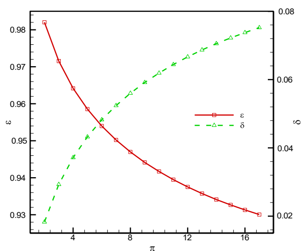
Figure 12 Variation of the fuel flow saving ratio and the multiplication ratio of fuel heat sink with the cycle pressure ratio
