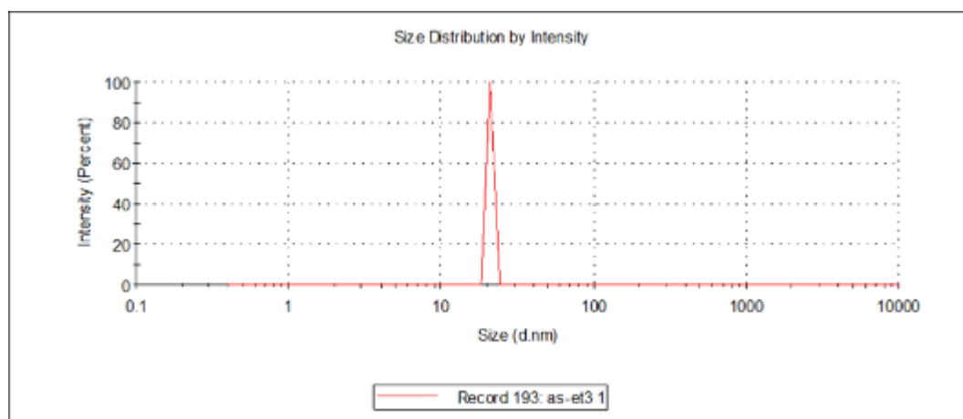
Figure 8 Dynamic Light Scattering (DLS) analysis of synthesized ZnO NPs of Andrographis alata ethanol extract
