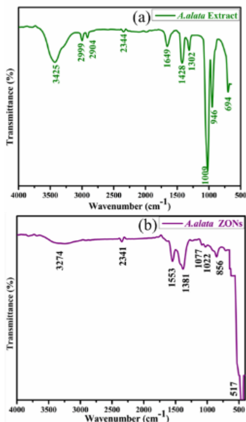
Figure 7 Fourier Transform Infrared (FTIR) spectra of Andrographis alata (a) ethanol extract and (b) synthesized ZONs.
