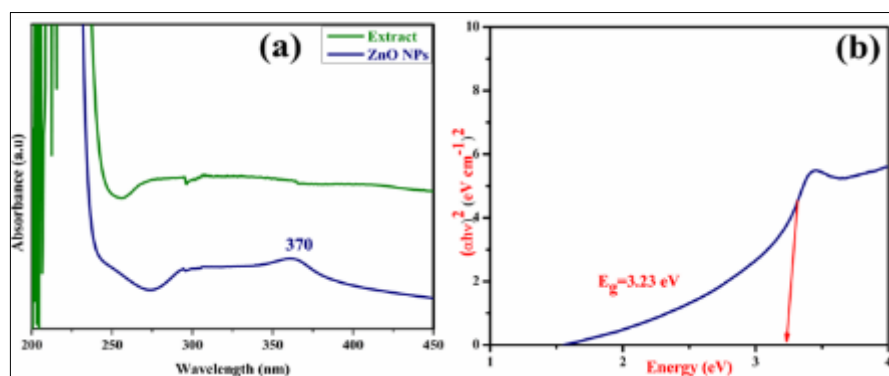
Figure 1 UV-Vis spectra of Andrographis alata (a) ethanol extract and synthesized ZONs and (b) Tauc plot
