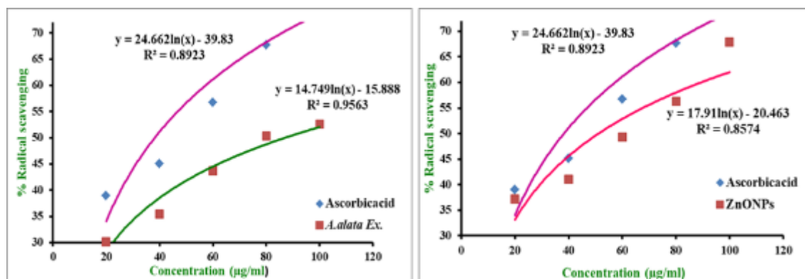
Figure 11 DPPH Radical scavenging percent of Andrographis alata ethanol extract and synthesized ZONs
