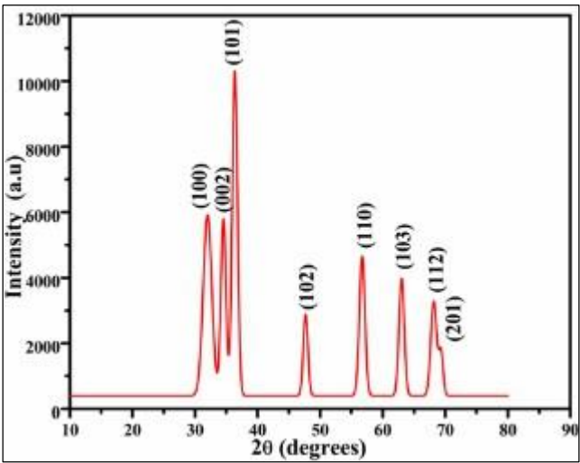
Figure 4 X-ray Diffraction pattern of ZONs synthesized from Andrographis alata ethanol extract
