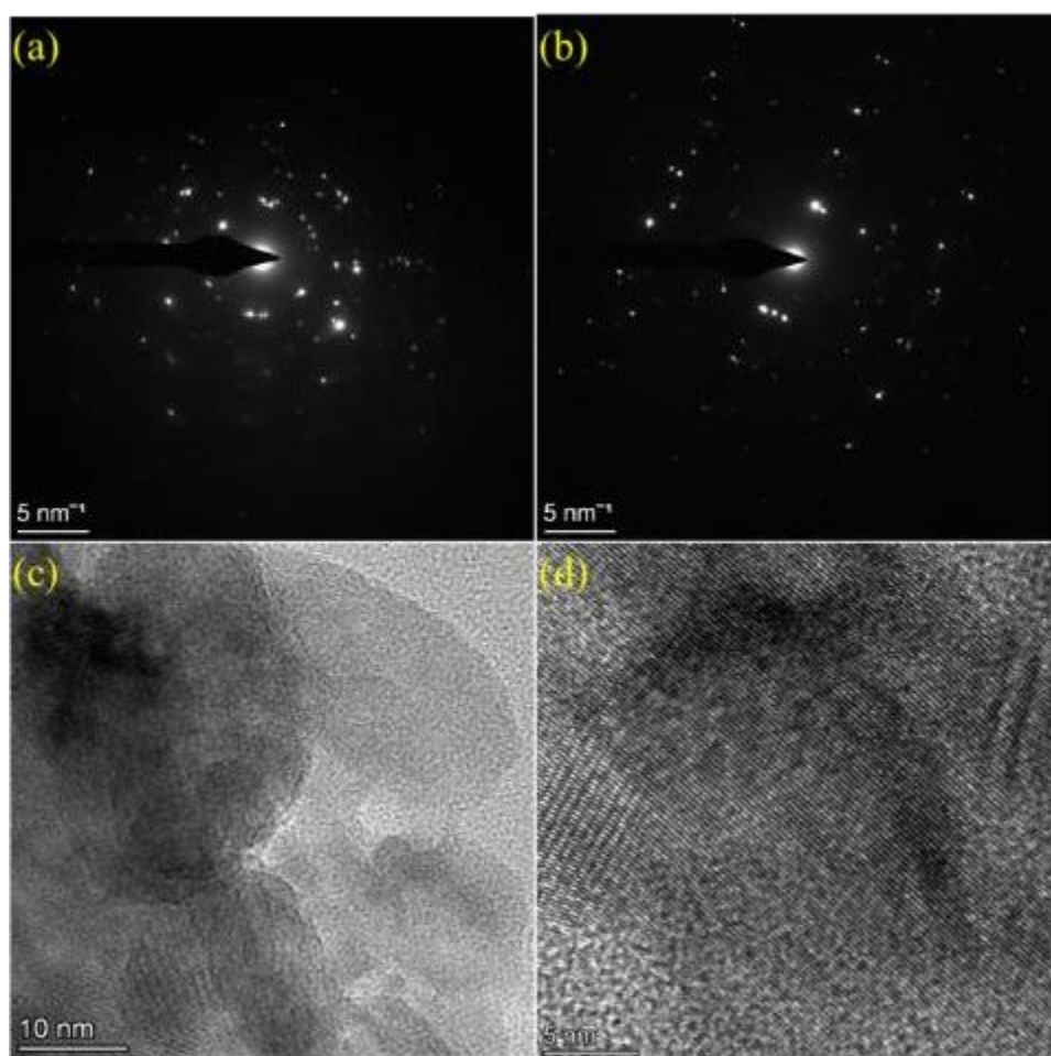
Figure 6 SAED of Andrographis alata ZONs: (a) polycrystalline, (b) single crystalline, and planes on crystalline grains (c) in 10nm and (d) in 5nm
