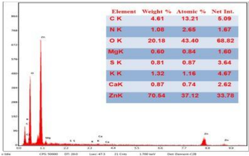
Figure 3 Energy Dispersive X-ray (EDAX) spectra of ZONs from Andrographis alata ethanol extract
