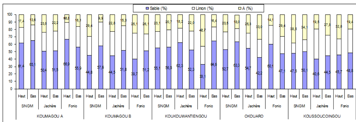
Figure 2 Dynamics of coarse elements in soils at study sites
