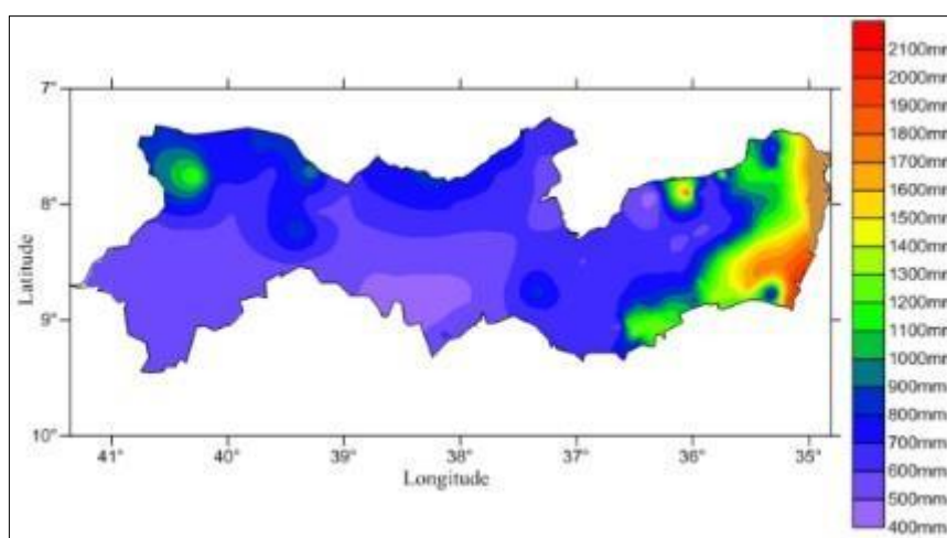
Figure 2 Annual rainfall (mm) for the period between 30 and 100 years with observations for the state of Pernambuco
