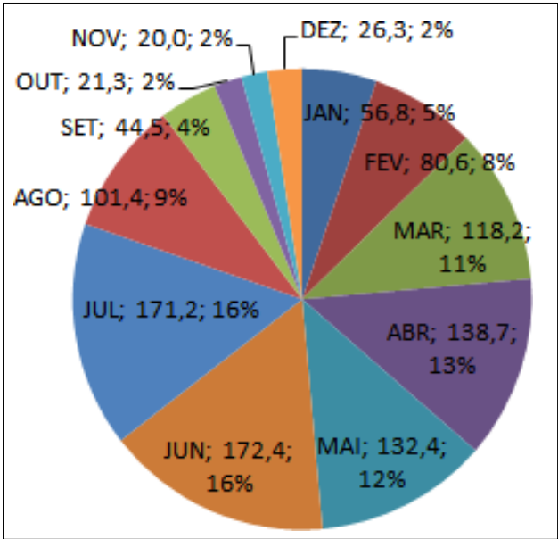
Figure 4 Distribution of monthly rainfall (mm) and its percentage values in the period 1981-2020 in the municipality of Lagoa Seca - PB
