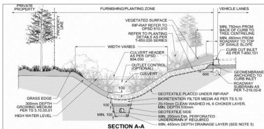
Figure 1 A cross-sectional diagram of a typical bioswale, detailing its structural components
