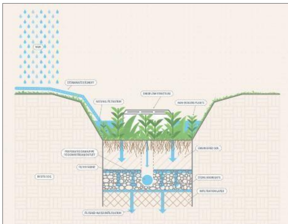
Figure 2 A flow path diagram demonstrating how stormwater moves through a bioswale system
