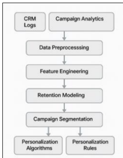
Figure 2 Data pipeline for customer retention modeling and campaign personalization. This pipeline illustrates the integration of multi-source data inputs such as CRM logs and campaign analytics through stages of data preprocessing, feature engineering, and retention modeling. The output guides campaign segmentation, which informs both personalization algorithms and rules, enabling real-time, targeted outreach strategies
