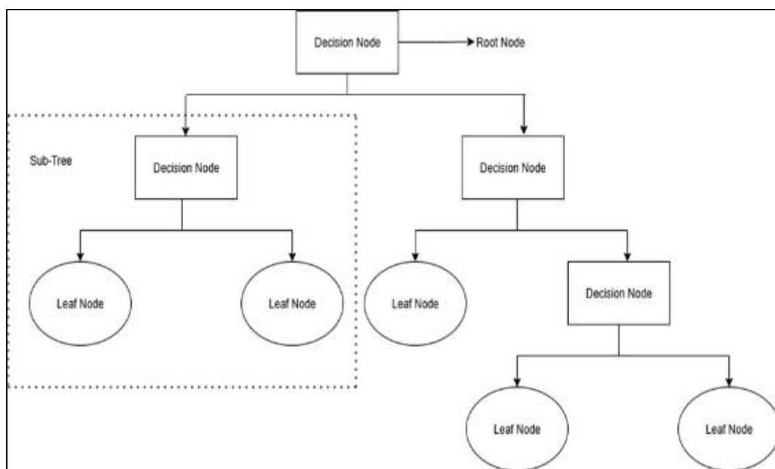
Figure 2 Decision Tree
