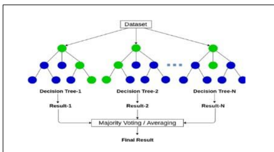
Figure 3 Random Forest
