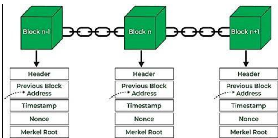
Figure 1 Blockchain Technology
