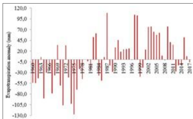
Figure 12 Distribution of the annual evapotranspiration anomaly for the municipal area of Santa Filomena - PI in the period 1960 - 2017
