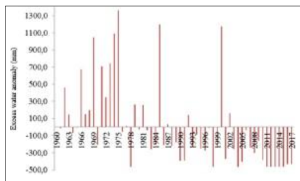
Figure 32 Representativeness of annual water surplus anomalies for the municipal area of Santa Filomena-PI in the period 1960-2017
