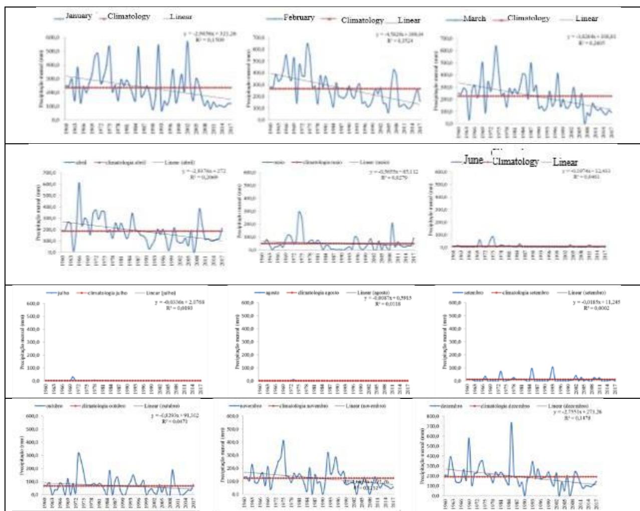
Figure 7 Time distribution of linear regression of monthly rainfall from January to December in the period from 1960 to 2017 for the municipality of Santa Filomena - PI
