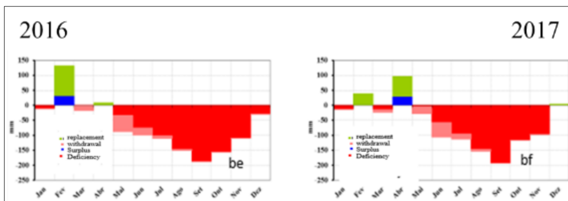
Figure 27 ac Representatives of the annual water balance of 2016(be) and 2017(bf) for the municipal area of Santa Filomena-PI
