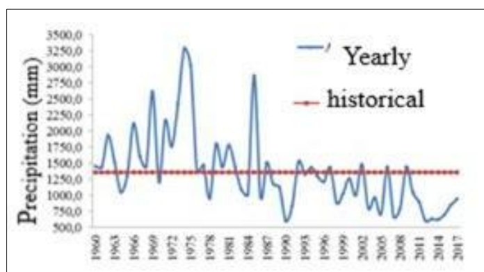
Figure 4 Distribution of annual and historical average precipitation for the municipal area of Santa Filomena - PI in the period 1960-2017
