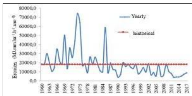
Figure 24 Annual variability of erosivity in the period 1960-2017 in the area of the municipality of Santa Filomena - PI
