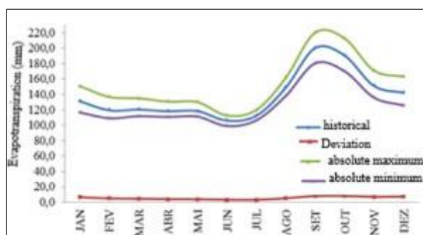
Figure 13 Distribution of monthly evapotranspiration and its absolute maximum and minimum values and standard deviation for the municipal area of Santa Filomena - PI in the period 1960 - 2017
