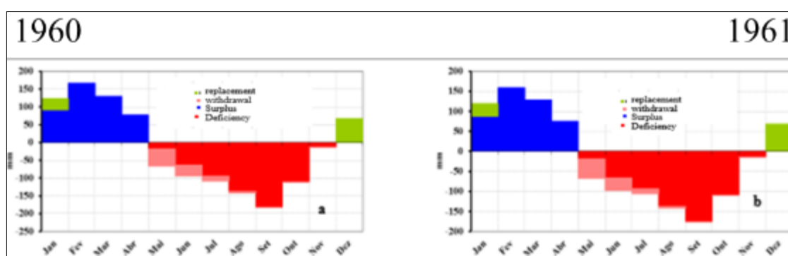
Figure 27 a Representatives of the annual water balance of 1960(a) and 1961(b) for the municipal area of Santa Filomena-PI
