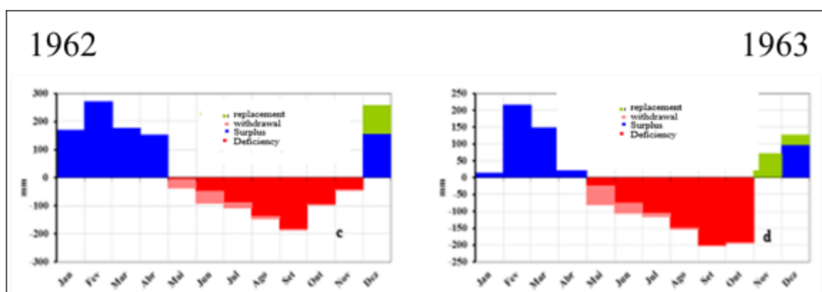
Figure 27 b Representatives of the annual water balance of 1962(c) and 1963(d) for the municipal area of Santa Filomena-PI
