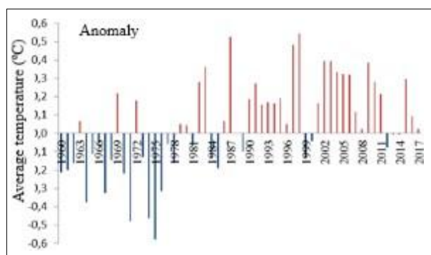
Figure 18 Average annual air temperature anomaly for the municipal area of Santa Filomena-PI in the period 1960-2017
