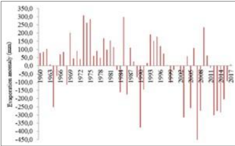
Figure 16 Distribution of the annual evaporation anomaly for the municipal area of Santa Filomena-PI in the period 1960-2017
