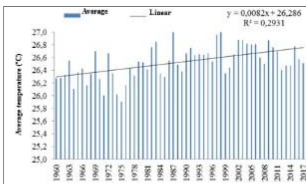
Figure 19 Distribution of the average annual air temperature and its lineares trend for the municipal area of Santa Filomena-PI in the period 1960-2017
