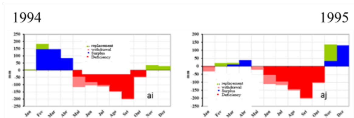
Figure 27 r Representatives of the annual water balance of 1994(ai) and 1995(aj) for the municipal area of Santa Filomena-PI
