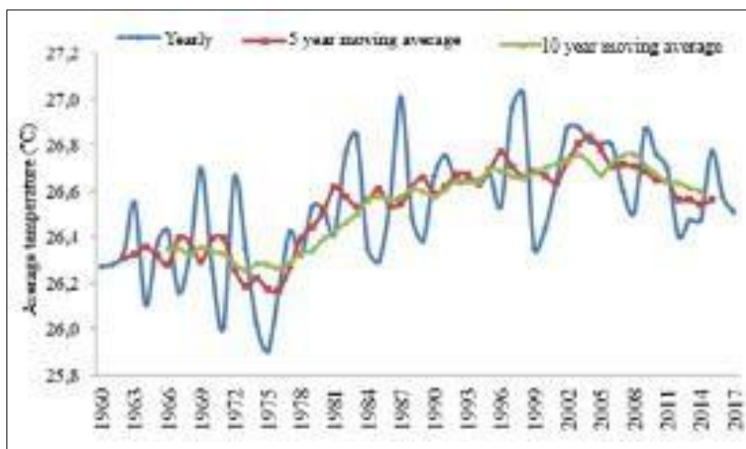
Figure 20 Distribution of the annual average temperature and its moving averages for 5 and 10 years for the municipal area of Santa Filomena-PI in the period 1960-2017
