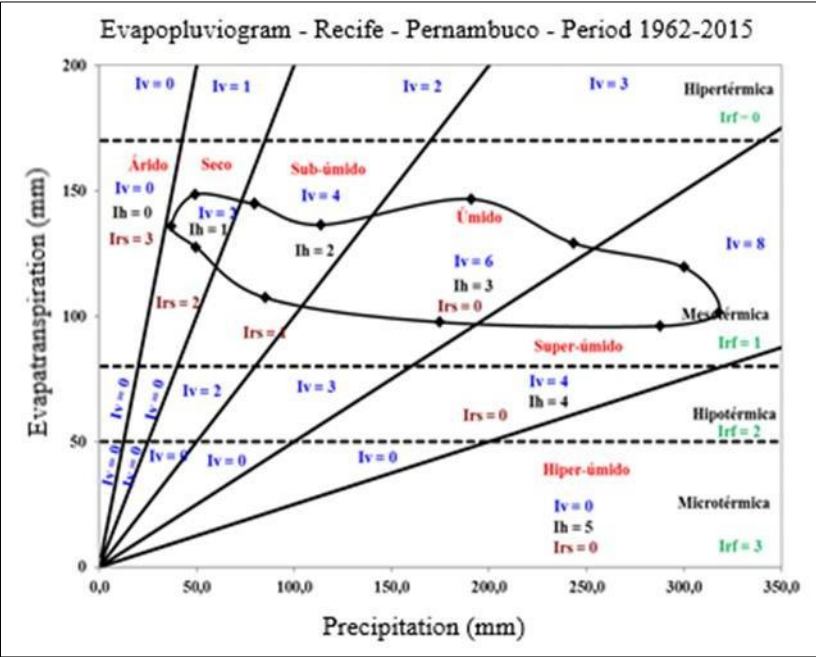
Figure 3 Distribution of water sectors and thermal bands of the evapopluvigram Recife – PE
