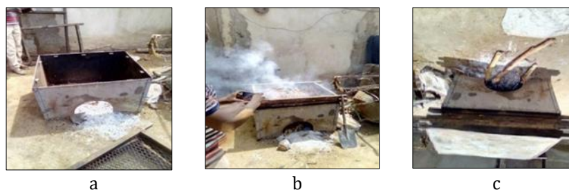
Figure 2 Smoking process with the PRESIBAL kiln, a) PRESIBAL kiln; b and c) fish being smoked
