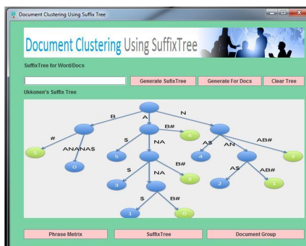
Figure 8 Document clustering
