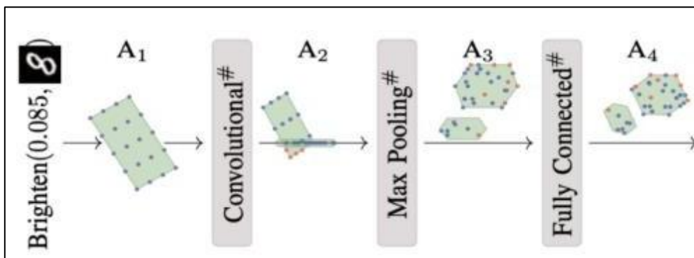
Figure 5 Abstraction algorithm (Adapted from https://www.cs.utexas.edu/~swarat/pubs/sp2018-ai2.pdf )
