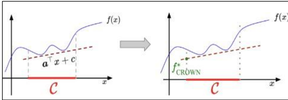
Figure 3 Global lower bound with Crown (Adapted from https://arxiv.org/pdf/2103.06624 )
