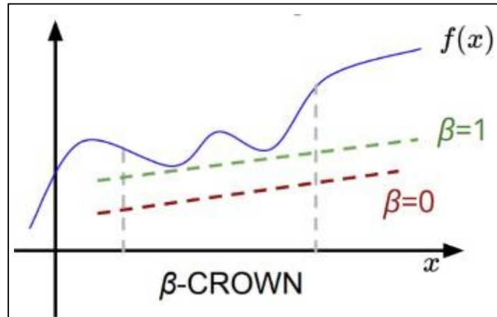
Figure 4 Global lower bound with Beta-Crown (Adapted from https://arxiv.org/pdf/2103.06624 )
