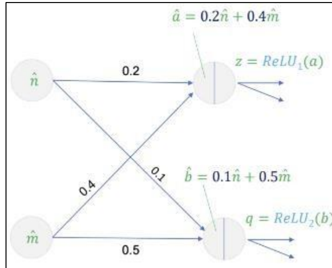
Figure 6 Representation of affine transformation
