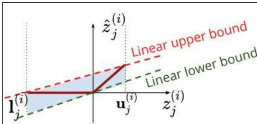
Figure 2 Lower and Upper bounds on ReLU (Adapted from https://arxiv.org/pdf/1811.00866 )
