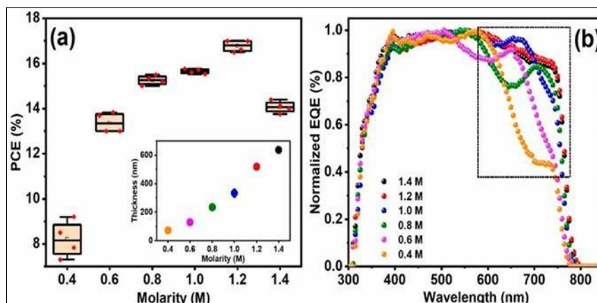
Figure 2 Concentration-dependent Perovskite solar cell performance. Inset depicts perovskite concentration-dependent thickness. Equal-weighted-element spectra
