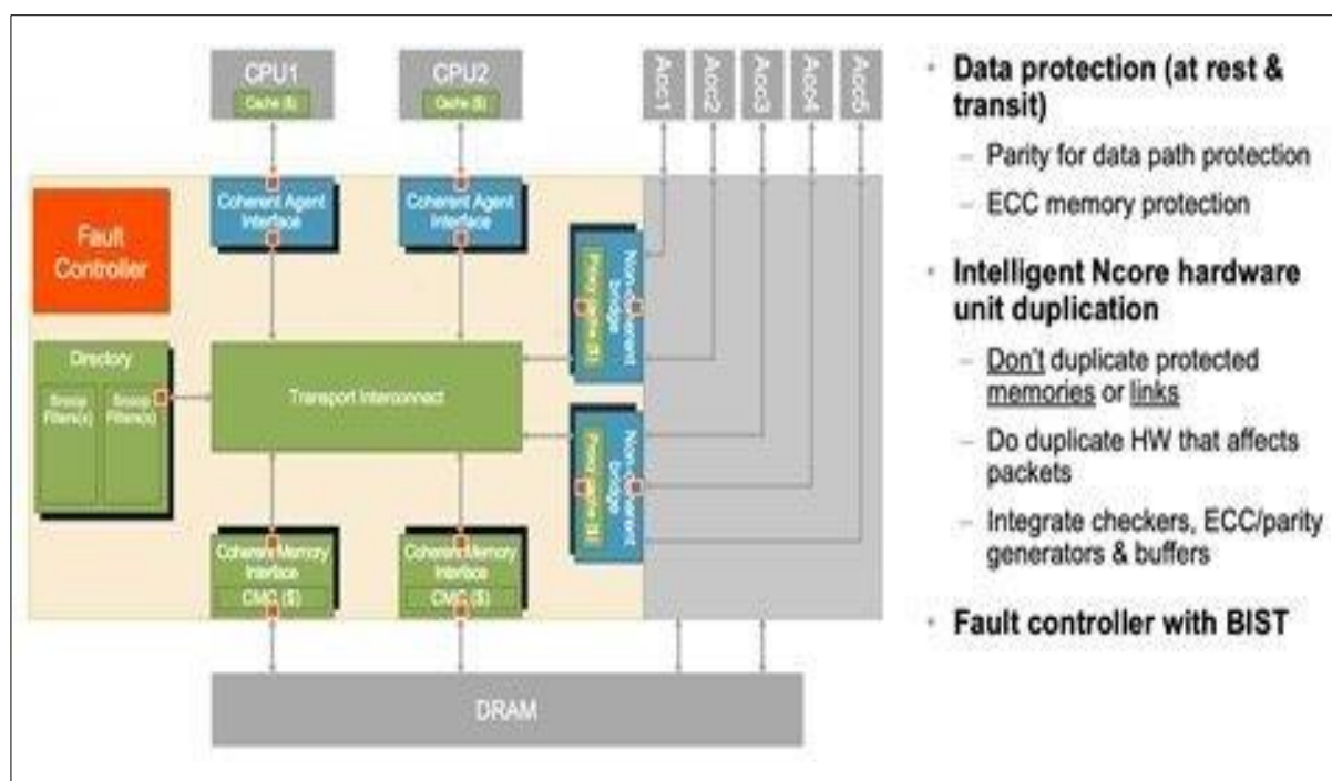
Figure 4 Re-Architecting SoCs for the AI Era
