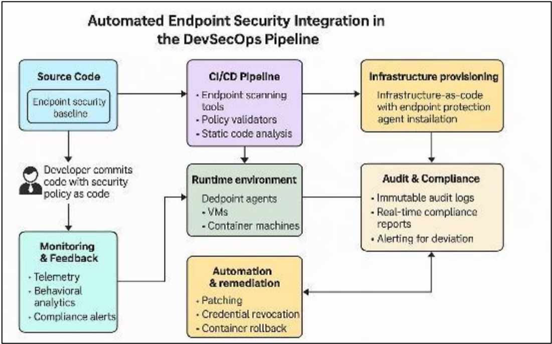
Figure 3 Automated Endpoint Security Integration in DevSecOps Lifecycle: From Threat Detection to Compliance
