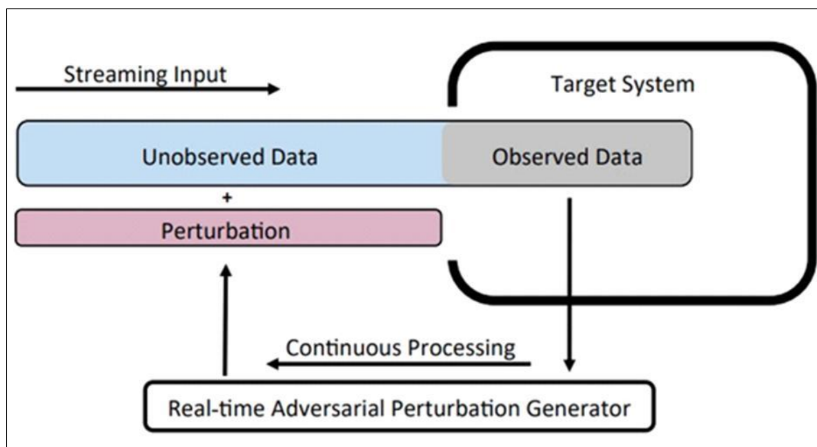
Figure 3 Illustration of the real-time adversarial attack scheme
