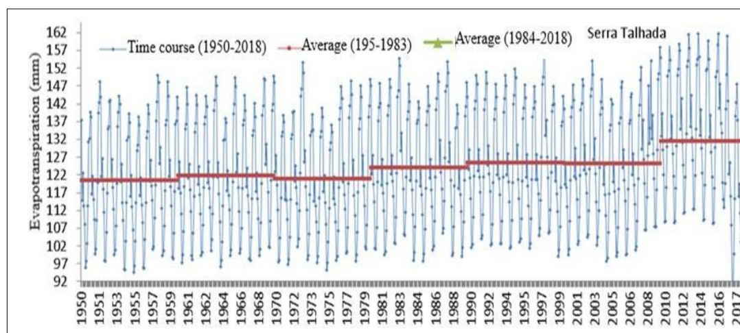
Figure 7 Variability of evapotranspiration between the years 1950-2018 and decadal averages (1950-1959; 1960-1969; 1970-1979; 1980-1989; 1990-1999; 2000-2009; 2010-2018) in the municipality of Serra Carved – PE
