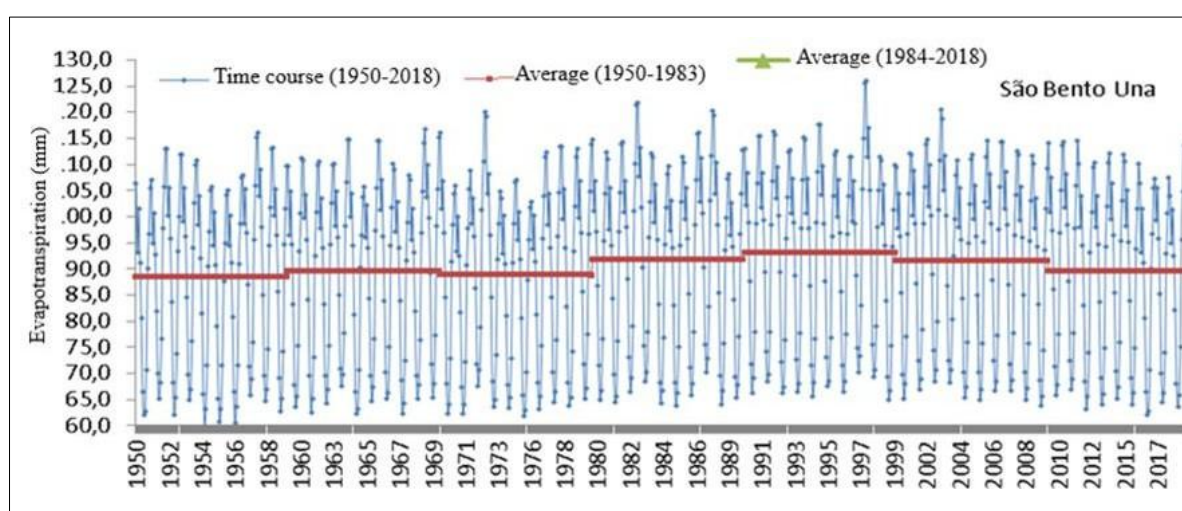
Figure 6 Variability of evapotranspiration between the years 1950-2018 and decadal averages (1950-1959; 1960-1969; 1970-1979; 1980-1989; 1990-1999; 2000-2009; 2010-2018) in the municipality of São Bento do Una – PE.
