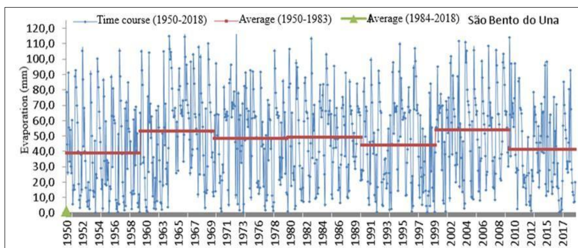
Figure 8 Variability of evaporation between the years 1950-2018 and decadal averages (1950-1959; 1960-1969; 1970-1979; 1980-1989; 1990-1999; 2000-2009; 2010-2018) in the municipality of São Bento do Una – PE
