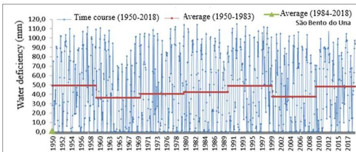
Figure 10 Variability of water deficit between the years 1950-2018 and decadal averages (1950-1959; 1960-1969; 1970-1979; 1980-1989; 1990-1999; 2000-2009; 2010-2018) in the municipality of São Bento do Una – PE
