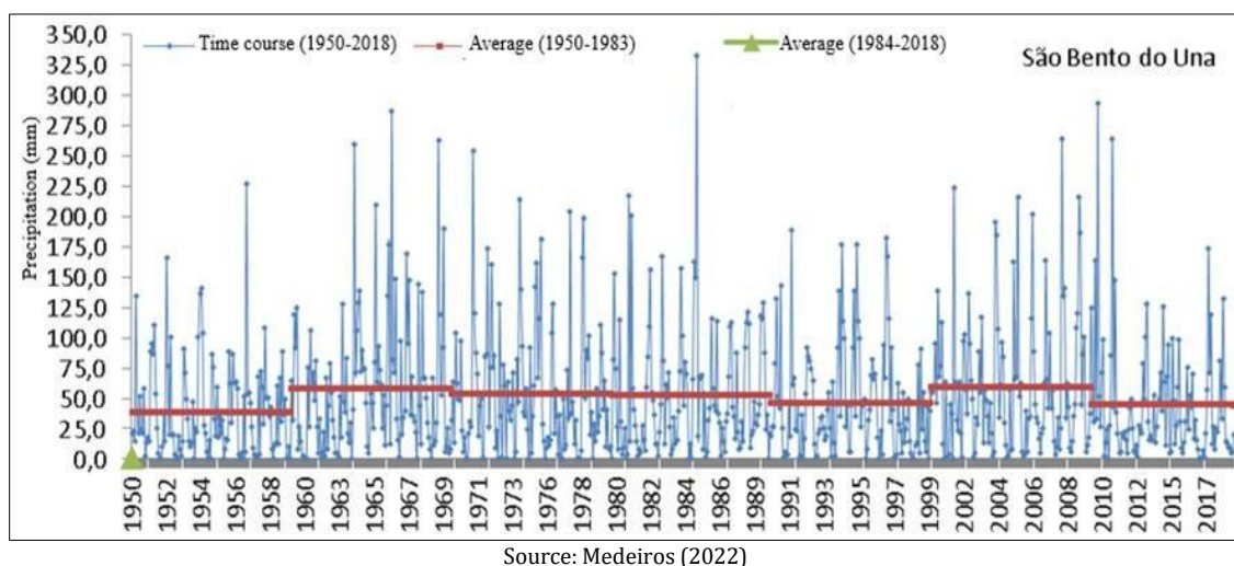
Figure 4 Variability of rainfall between the years 1950-2018 and decadal averages (1950-1959; 1960-1969; 1970-1979; 1980-1989; 1990-1999; 2000-2009; 2010-2018) in the municipality of São Bento do Una – PE
