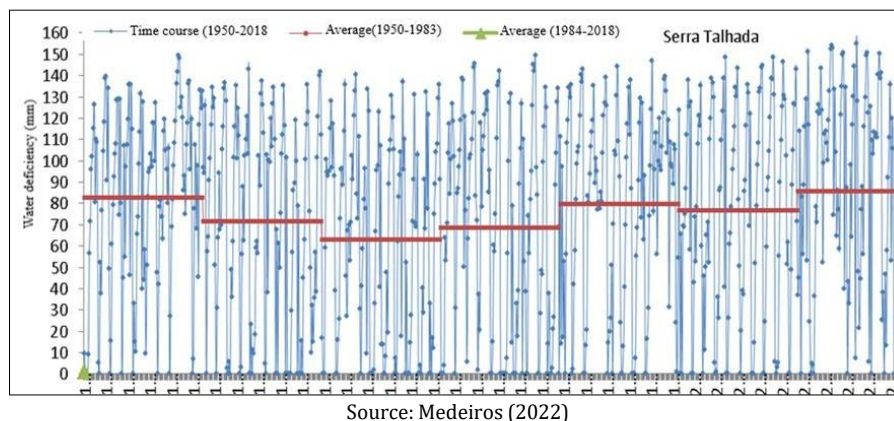
Figure 11 Water deficit variability between the years 1950-2018 and decadal averages (1950-1959; 1960-1969; 1970-1979; 1980-1989; 1990-1999; 2000-2009; 2010-2018) in the municipality of Serra Talhada - PE
