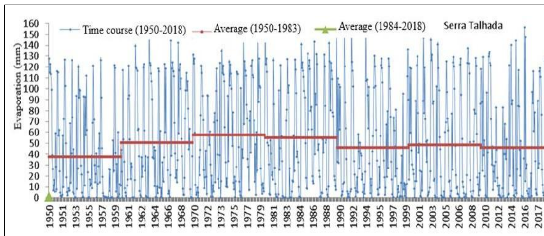
Figure 9 Variability of evaporation between the years 1950-2018 and decadal averages (1950-1959; 1960-1969; 1970-1979; 1980-1989; 1990-1999; 2000-2009; 2010-2018) in the municipality of Serra Carved – PE
