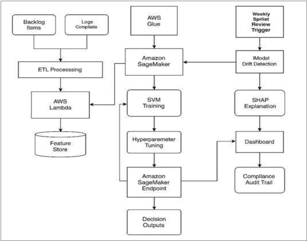
Figure 2 Data architecture integrating AWS, ML model, and feedback loop
