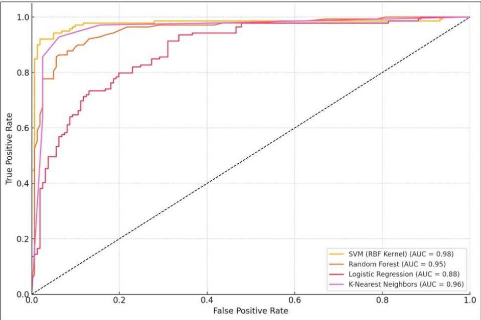
Figure 3 ROC-AUC curves comparing ML models
