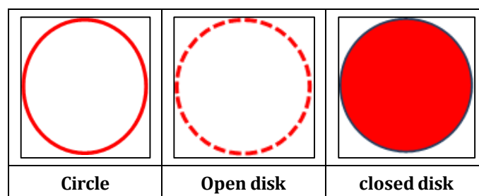
Figure 1 Circle, open and closed disk
