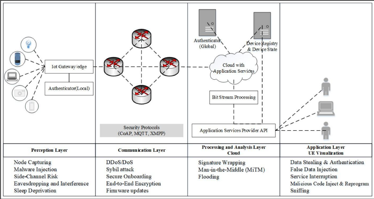
Figure 2 Layered view of IoT for AA and Security Risks [50]
