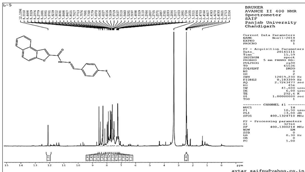
Figure 2 ^1\text{H} NMR Spectrum of Ligand L
