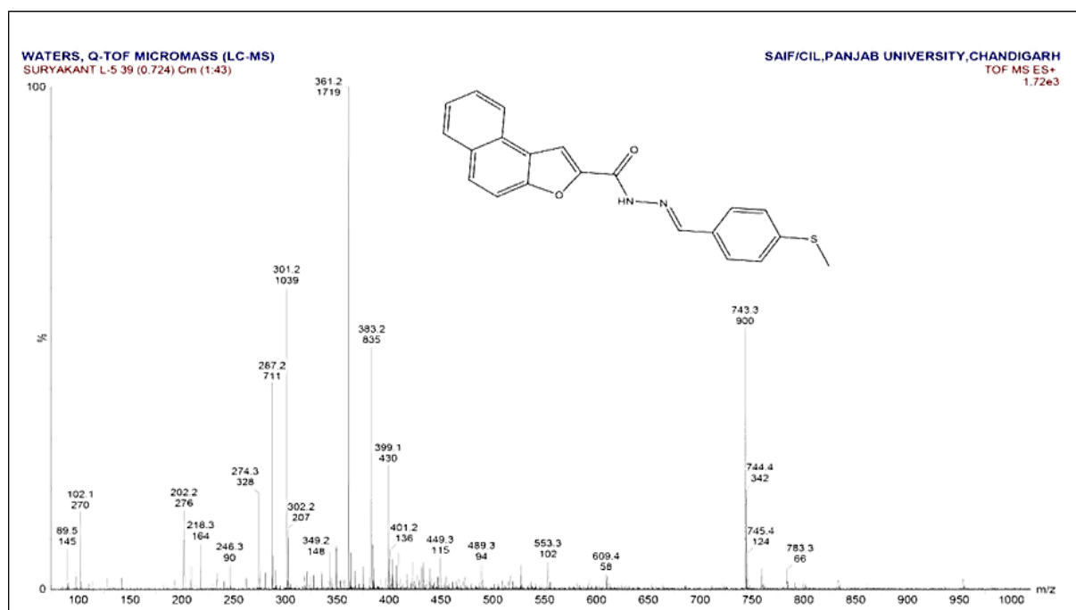
Figure 3 ^1\text{Mass} Spectra of the ligand (L)
